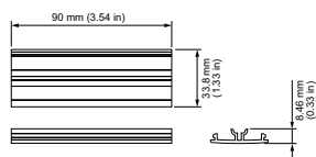
Mounting Track
