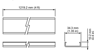
Mounting Track
