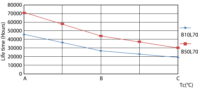
LEDtube_70K_LifetimeVsTc-LED
