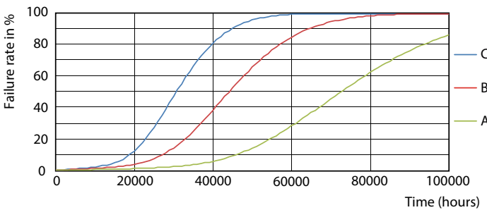
LEDtube_70K_FailureRate-LED
