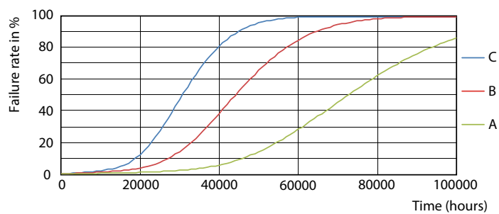
LEDtube_70K_FailureRate-LED
