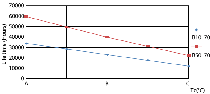
LEDtube_60K_LifetimeVsTc
