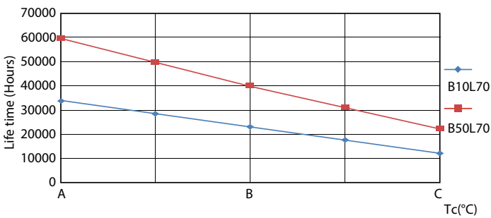
LEDtube_60K_LifetimeVsTc
