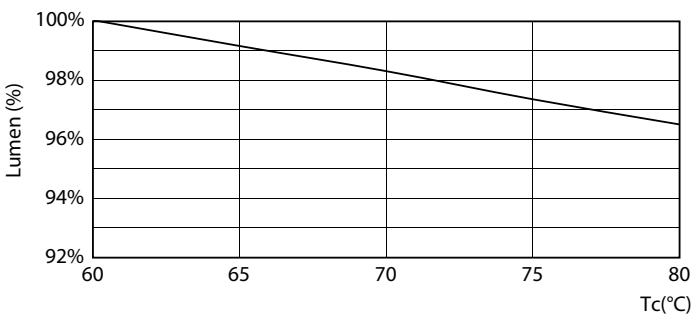
LEDtube MAS 23W 60K LumenVsTc
