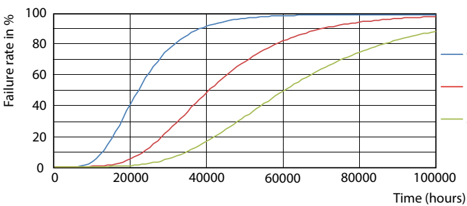
LEDtube_60K_FailureRate
