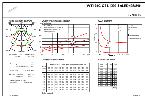
IFGU1_WT120CG2L12001xLED40S840
