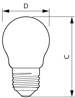
Bulb P45 40W 470lm 2700K E27 D FR
