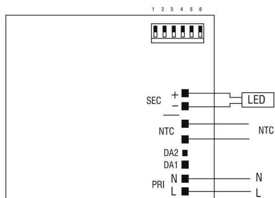
DALI diagram
