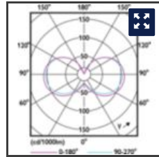
LEDcapsule MV 2,6W G9
