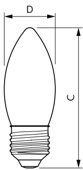
Candle B35 EU 3.5-40W 475lm WG E27 CL
