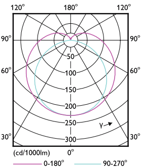
LEDtube MAS 13,5W G13 2500lm-LDD
