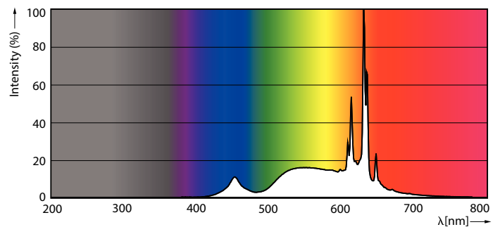
LEDbulb MAS SLR 7,2W A60 E27 927 CL-POC
