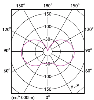
LEDbulb MAS SLR A60 7,2W E27 927 CL-LDD
