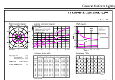
LEDbulb MAS SLR 10,5W A60 E27 927 CL-POC
