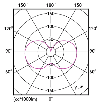
LEDbulb MAS SLR A60 10,5W E27 927 FR-LDD
