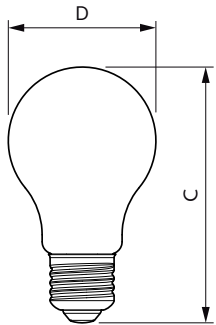
Bulb A60 EU 11.5-100W 1560lm WG E27 FR
