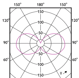
LEDcapsule CorePro 2W G9 827-LDD
