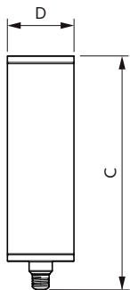
Bulb Crystal 230V 25W 270lm 1800K E27 D
