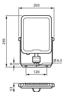
Ledinaire floodlight BVP105/106
