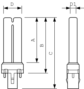
PL-S 5W/827/2P LM
