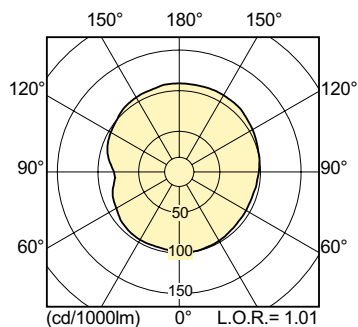
LDLD_CPO-TW_0005-Light distribution diagram
