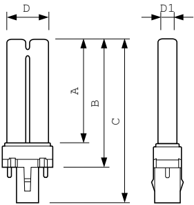
PL-S 9W/840/2P LM
