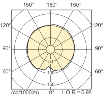
LDLD_CPO-TW_0002-Light distribution diagram
