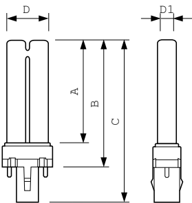
PL-S 11W/827/2P LM
