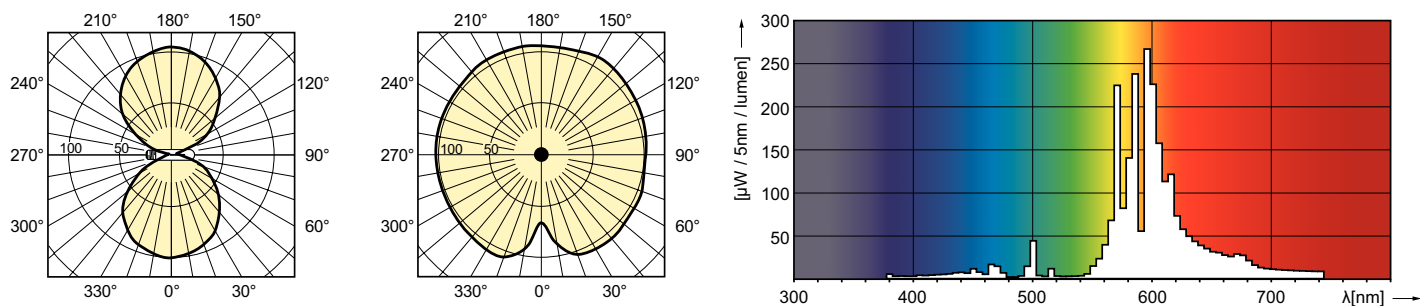
LDLD_SONTAPIA-Light distribution diagram
