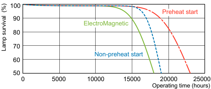
LDLE_TL-D9HLM_0002-Life expectancy diagram
