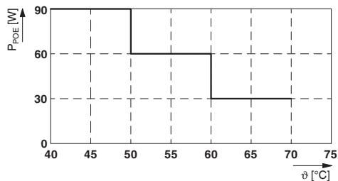
Derating pr. port
