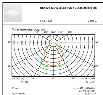
OFPC1_RC132VG4W60L60PSU1xLED34S830OC
