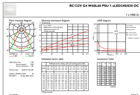
IFGU1_RC132VG4W60L60PSU1xLED34S830OC
