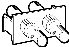
1U 2 ST SM/MM Dimensions: 23.9mm x 40.6mm x 42.4mm (.94"H x 1.6"W x 1.67"D) Shipping Weight: 28g (1 oz.)
