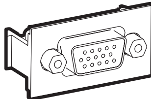
1U 15 Pin HD D- Sub Coupler SVGA Dimensions: 23.9mm x 40.6mm x 19mm (.94"H x 1.6"W x .75"D) Shipping Weight: 14g (.5 oz.)
