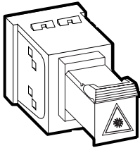
Simplex SC SM/MM Shuttered Dimensions: 23.9mm x 40.6mm x 27.4mm (.94"H x 1.6"W x 1.08"D) Shipping Weight: 14g (.5 oz.)
