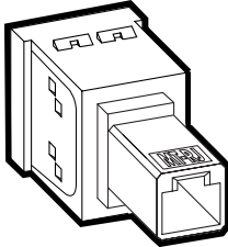
MT-RJ SM/MM Dimensions: 23.9mm x 17.8mm x 27.9mm (.94"H x .70"W x 1.1"D) Shipping Weight: 14g (.5 oz.)
