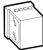
Single Position Blank Dimensions: 23.9mm x 17.8mm x 27.2mm (.94"H x .70"W x 1.07"D) Shipping Weight: 5.6g (.2 oz.)
