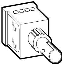
ST SM/MM Dimensions: 23.9mm x 40.6mm x 27.4mm (.94"H x 1.6"W x 1.08"D) Shipping Weight: 14g (.5 oz.)
