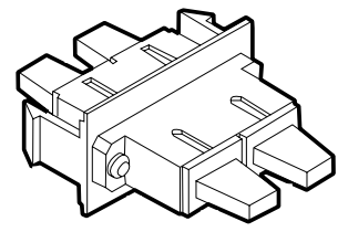
1U Duplex SC SM/MM Dimensions: 23.9mm x 40.6mm x 27.4mm (.94"H x 1.6"W x 1.08"D) Shipping Weight: 28g (1 oz.)
