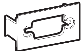
1U 15 Pin HD D- Sub Coupler Fascia Dimensions: 23.9mm x 40.6mm x 19mm (.94"H x 1.6"W x .75"D) Shipping Weight: 8.4g (.3 oz.)
