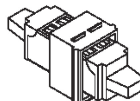
Duplex LC SM 23.5mm x 17.8mm x 25.7mm (.93"H x .70"W x 1.01"D) Shipping Weight: 12g (.43 oz.)
