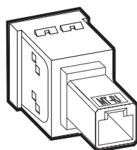
MT-RJ SM/MM 23.5mm x 17.8mm x 29.0mm (.93"H x .70"W x 1.14"D) Shipping Weight: 4.6g (.16 oz.)
