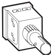
ST SM/MM 23.5mm x 17.8mm x 29.1mm (.93"H x .70"W x 1.15"D) Shipping Weight: 10.7g (.38 oz.)
