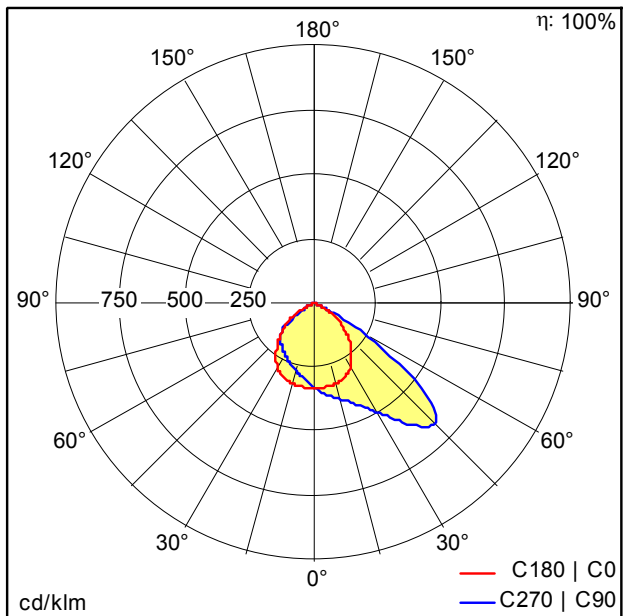
TE_LEO_LED_FL_IP66_210W_840_PC.Idt
