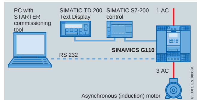
SINAMICS G110 configuration example (USS version with SIMATIC S7-200, PC inverter connection with optional PC inverter connection kit)
