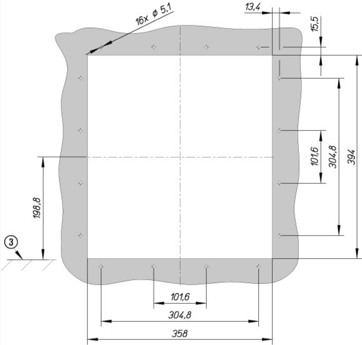
③ Top edge mounting floor of the Circuit Breaker
