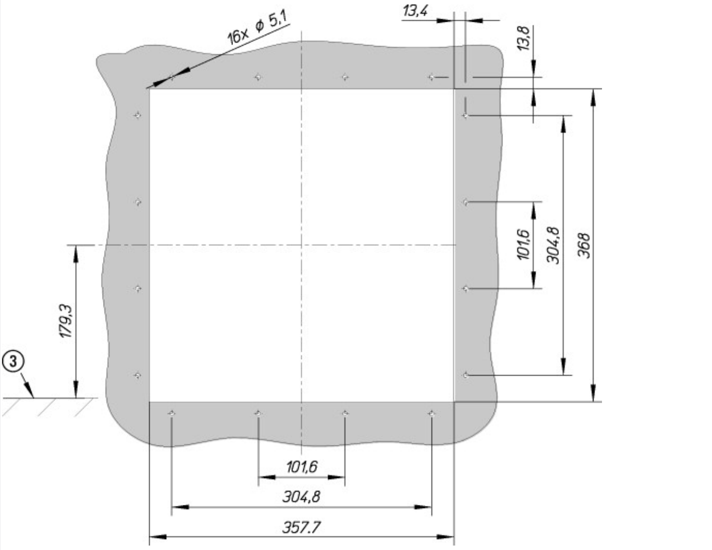
③ Top edge mounting floor of the Circuit Breaker
