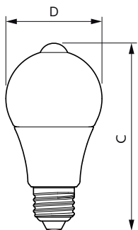
Bulb A60 220-240V 9-60W 806lm 4000K E27
