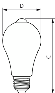
Bulb A60 220-240V 9-60W 806lm 2700K E27
