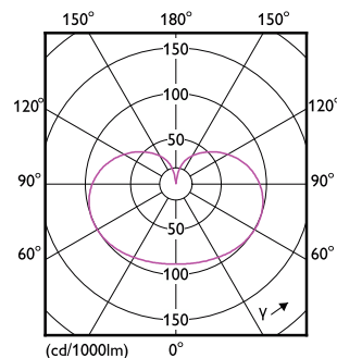
LEDbulb Sensor A60 8W E27 840 FR-LDD
