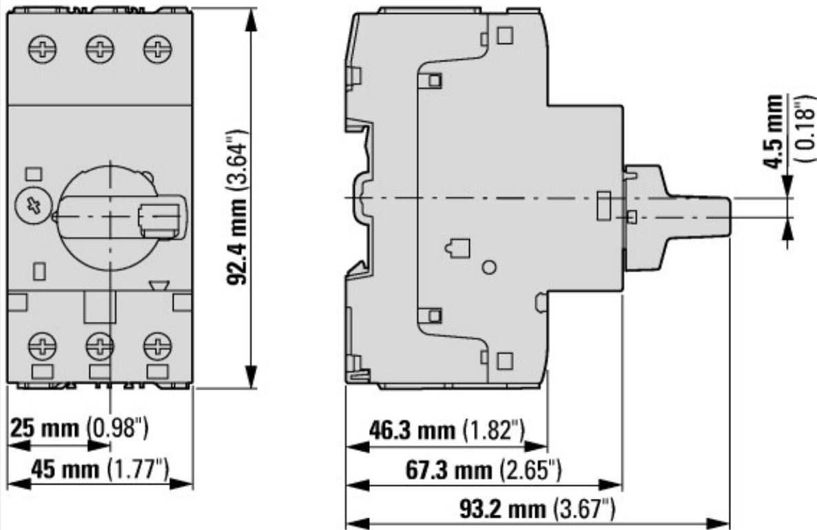
Motor-protective circuit-breakers with lockable rotary handles
