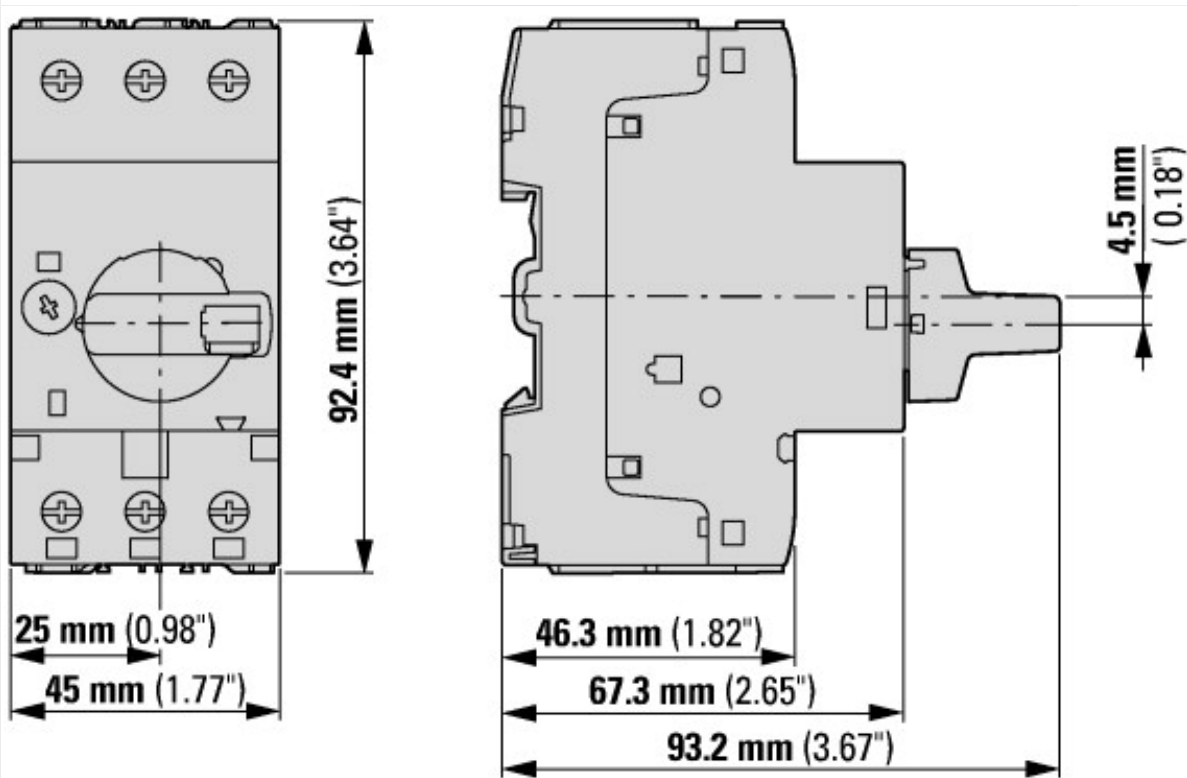
Motor-protective circuit-breaker with standard auxiliary contact PKZM0-...(+NHI-E-...-PKZ0) PKZM0-...-T(+NHI-E-...-PKZ0) PKM0-...(+NHI-E-...-PKZ0)
