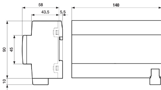
Dimension drawing
