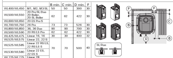
Safety distances with protective sheaths (all dimensions in millimeters)
