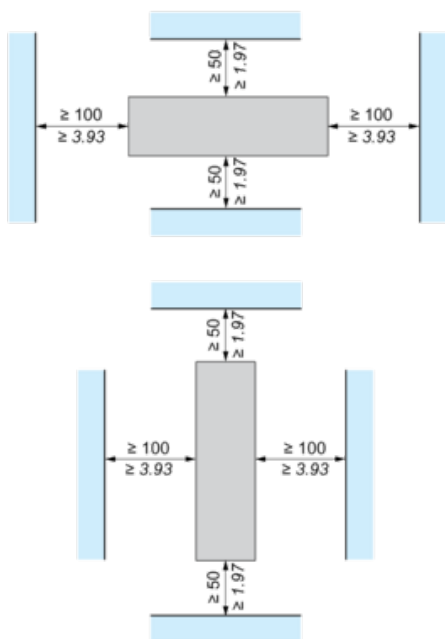
(1) Braking resistor
