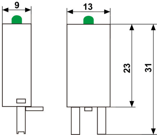
Dimensioned drawing: LED module green 24VAC/DC for S-Relay socket
