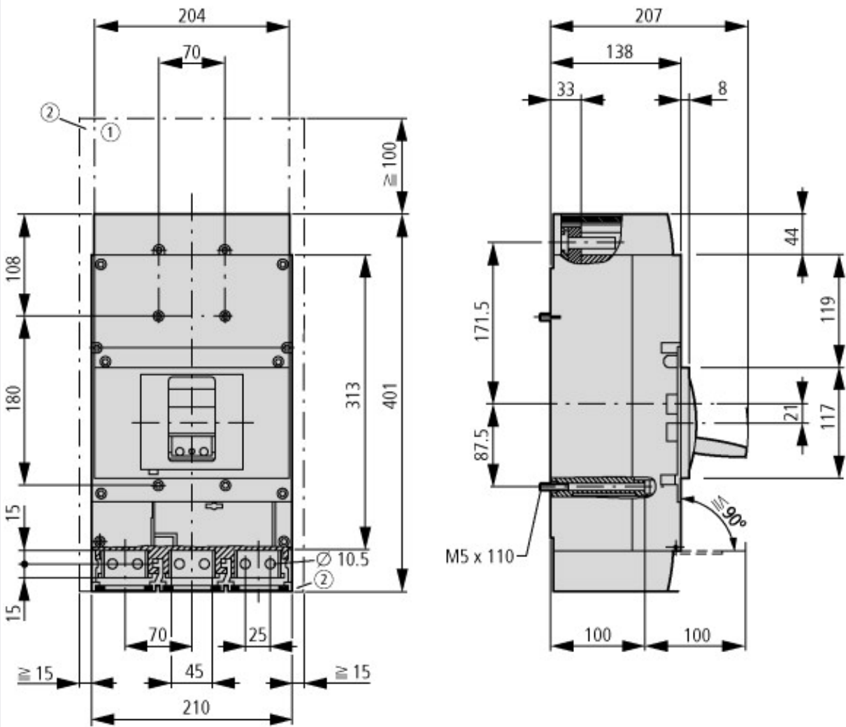
① Blow out area, minimum clearance to adjacent parts Ui ≤ 690 V: 100 mm Ui ≤ 1500 V: 200 mm ② Minimum clearance to adjacent parts Ui ≤ 1000 V: 15 mm Ui ≤ 1500 V: 70 mm
