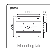
Mounting plate
