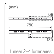
Linear 2-4 luminaires
