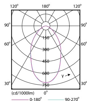
400W E40 Others ND 60D 840 4000K
