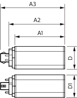
CorePro LED PLT HF 6.5W 840 4P GX24q-2
