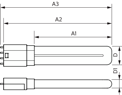
CorePro LED PLL HF 8W 840 4P 2G11
