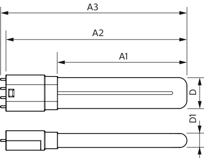
CorePro LED PLL EM/Mains 8W 830 4P
