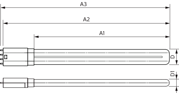
CorePro LED PLL EM/Mains 12W 830 4P
