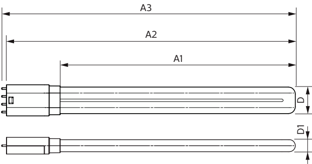
CorePro LED PLL Mains 24W 830 4P
