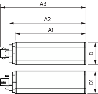
CorePro LED PLT HF 15W 840 4P GX24q-3
