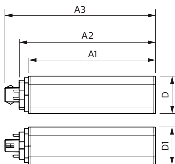
CorePro LED PLT HF 18.5W 830 4P GX24q-4
