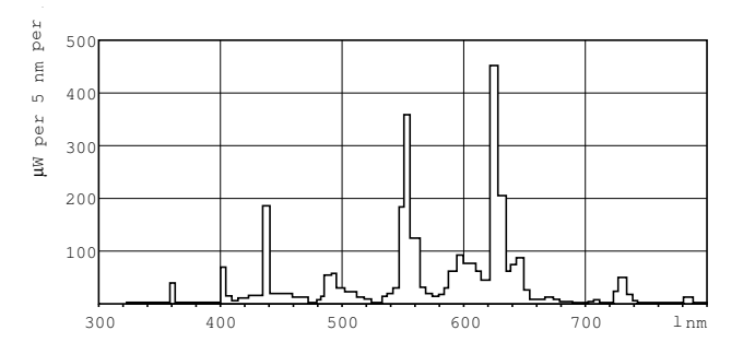
LDPB_TL5-HE8_830-Spectral power distribution B/W
